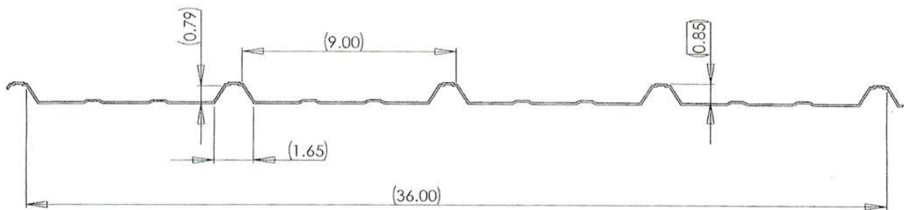
BOSS RIB PANEL PROFILE
