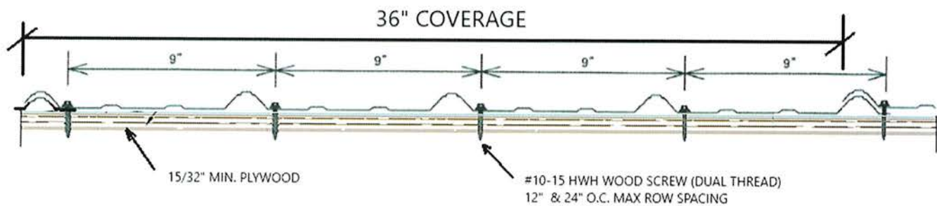
FASTENER PATTERN 12" OR 24" O.C.
